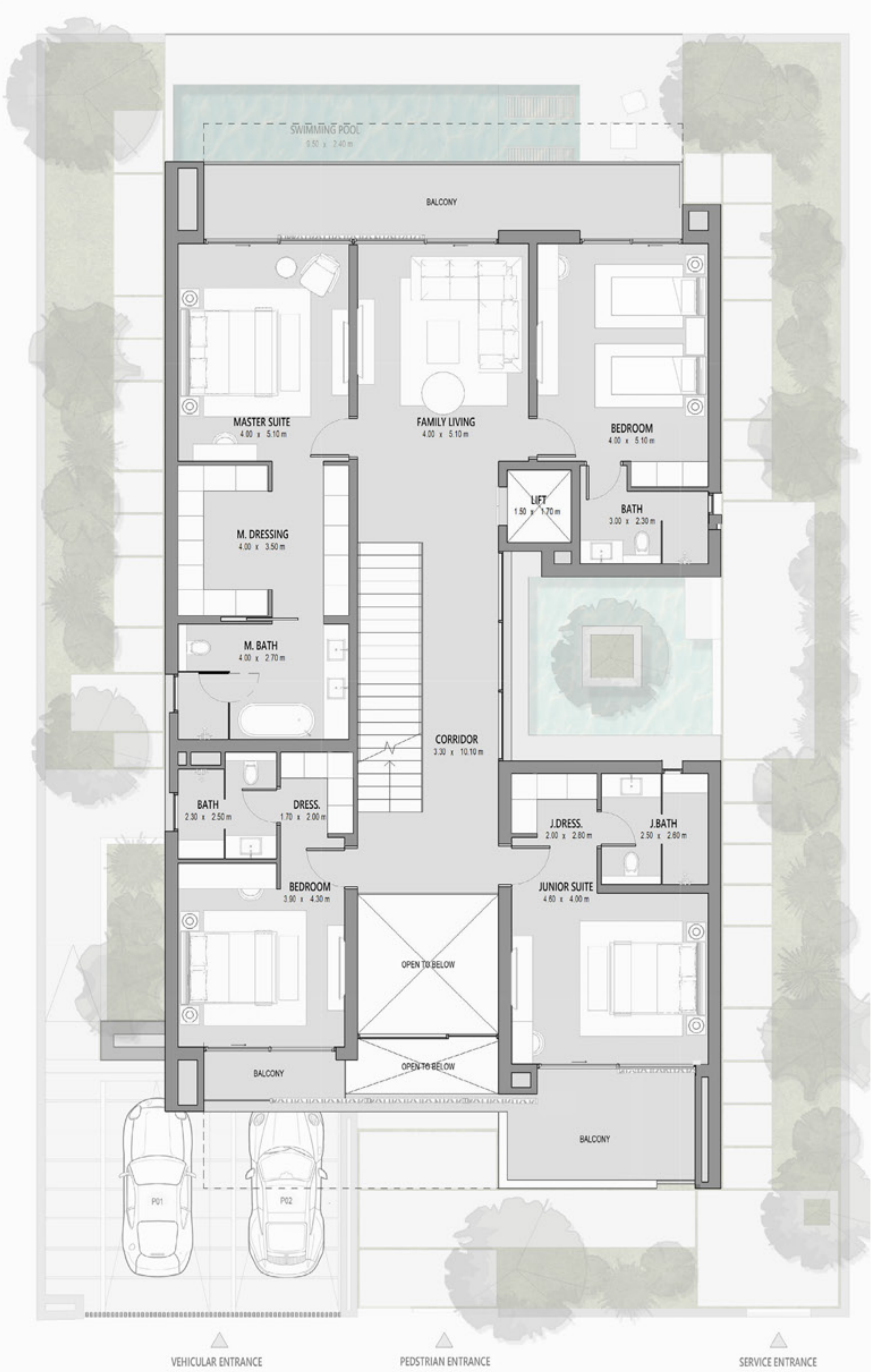
First Floor
