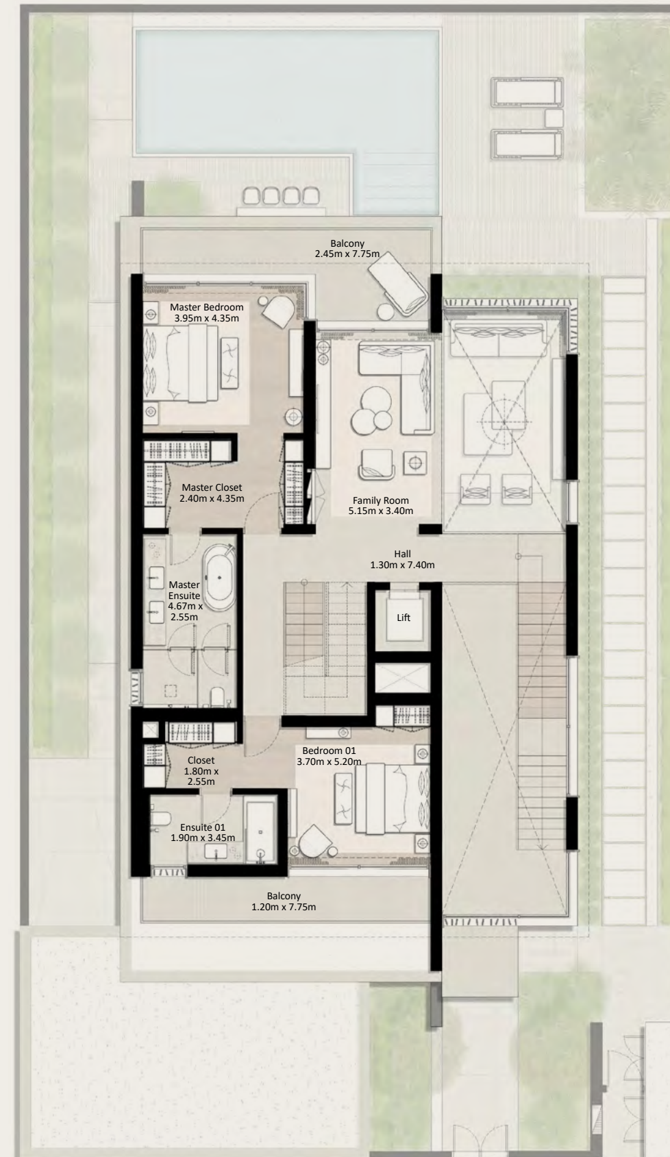
FIRST FLOOR
