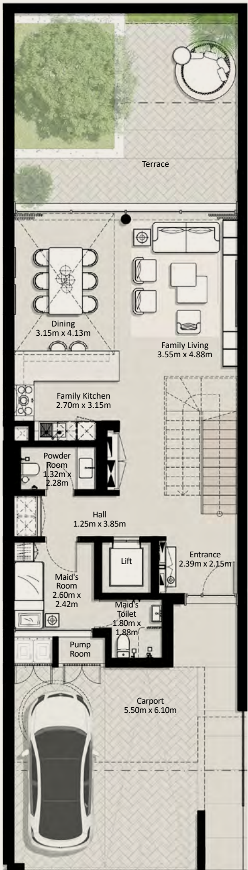
GROUND FLOOR
