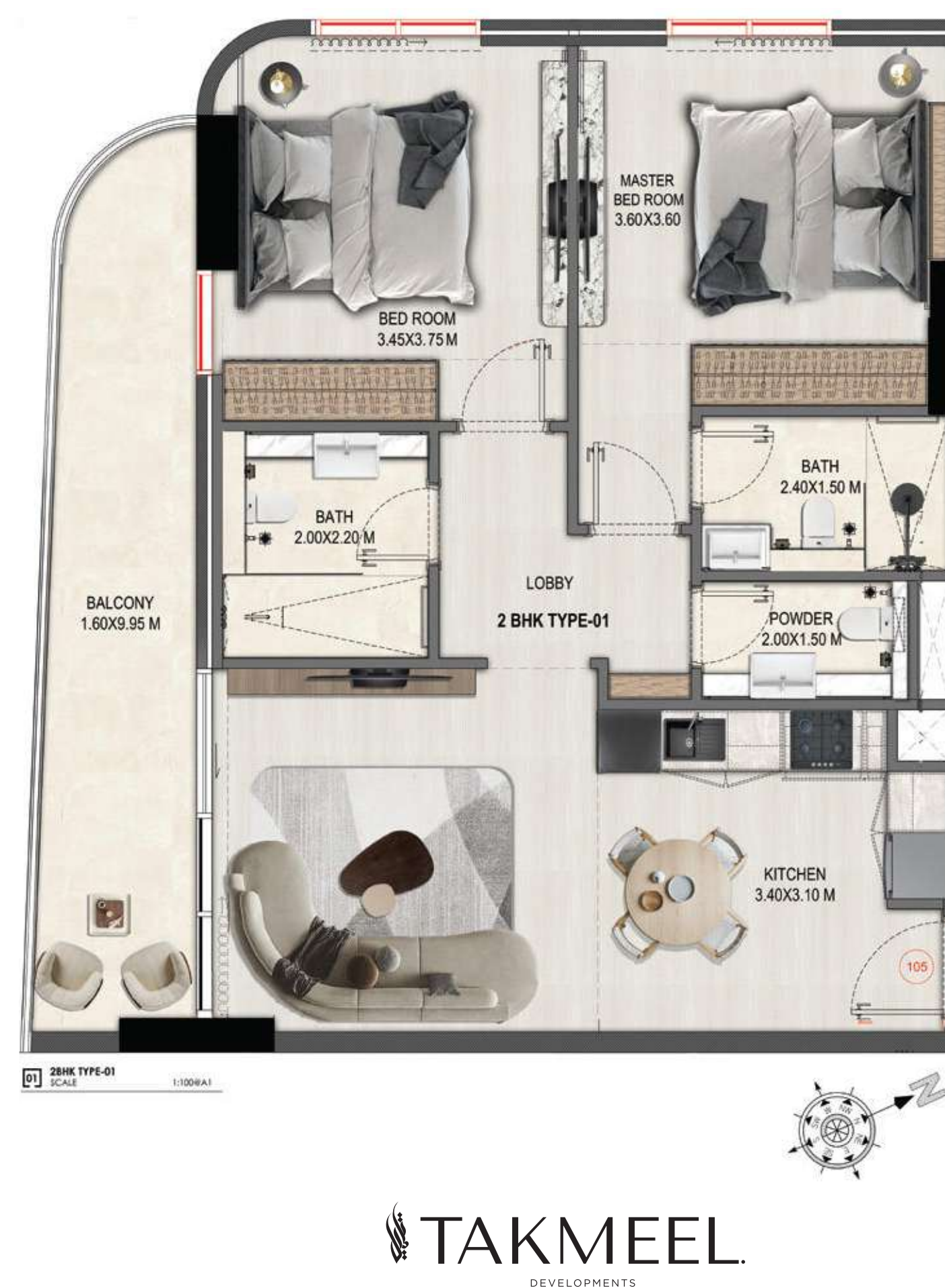
Unit Plan
