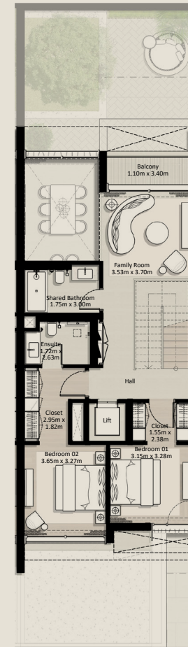
FIRST FLOOR
