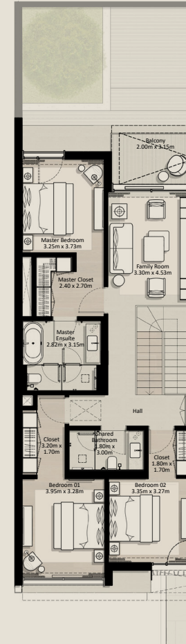
FIRST FLOOR
