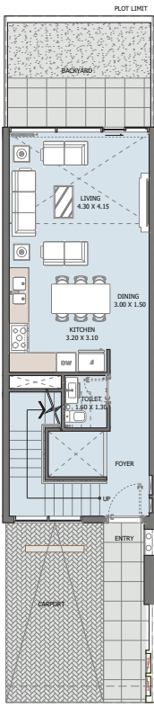
GROUND FLOOR
