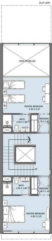
1ST FLOOR
