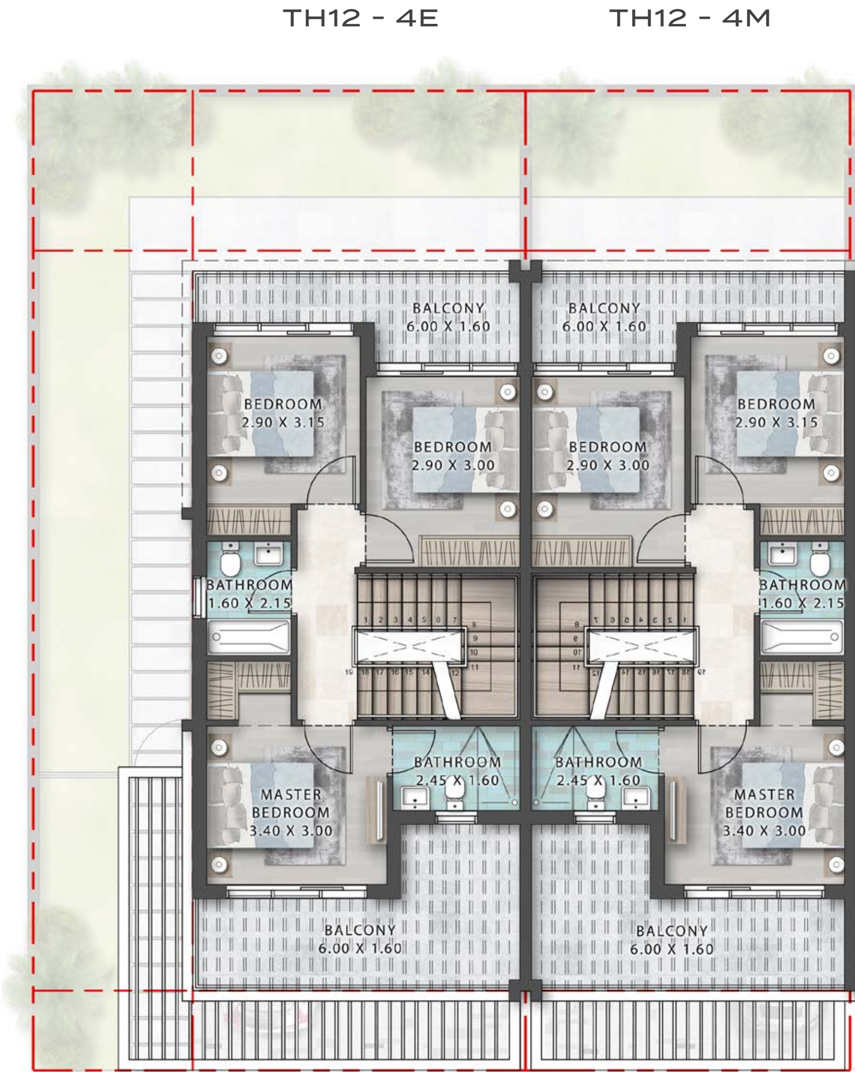
FIRST FLOOR
