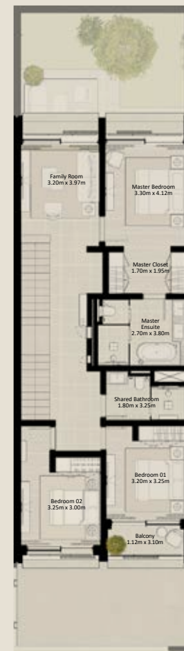
FIRST FLOOR
