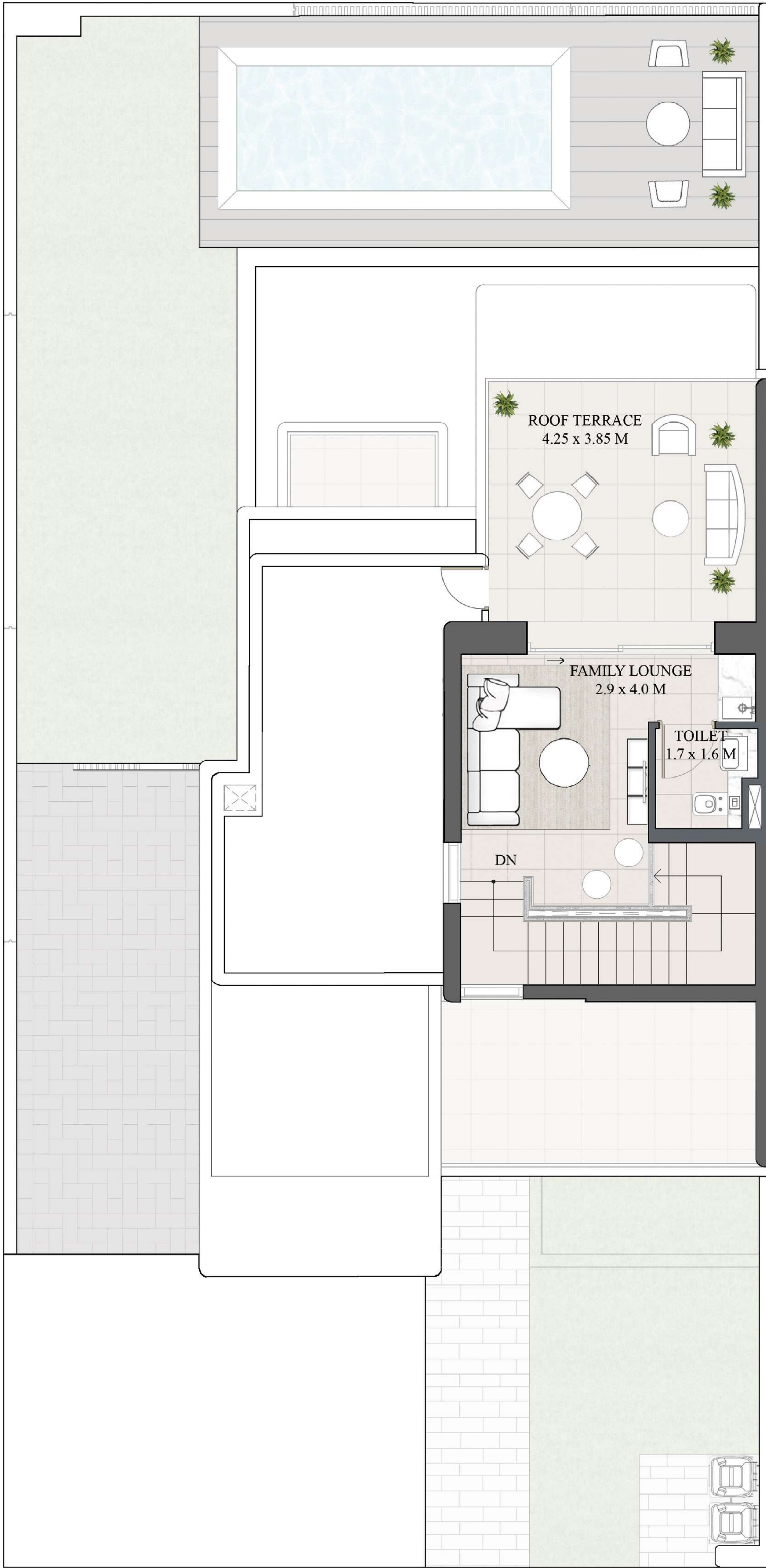
ROOF FLOOR
