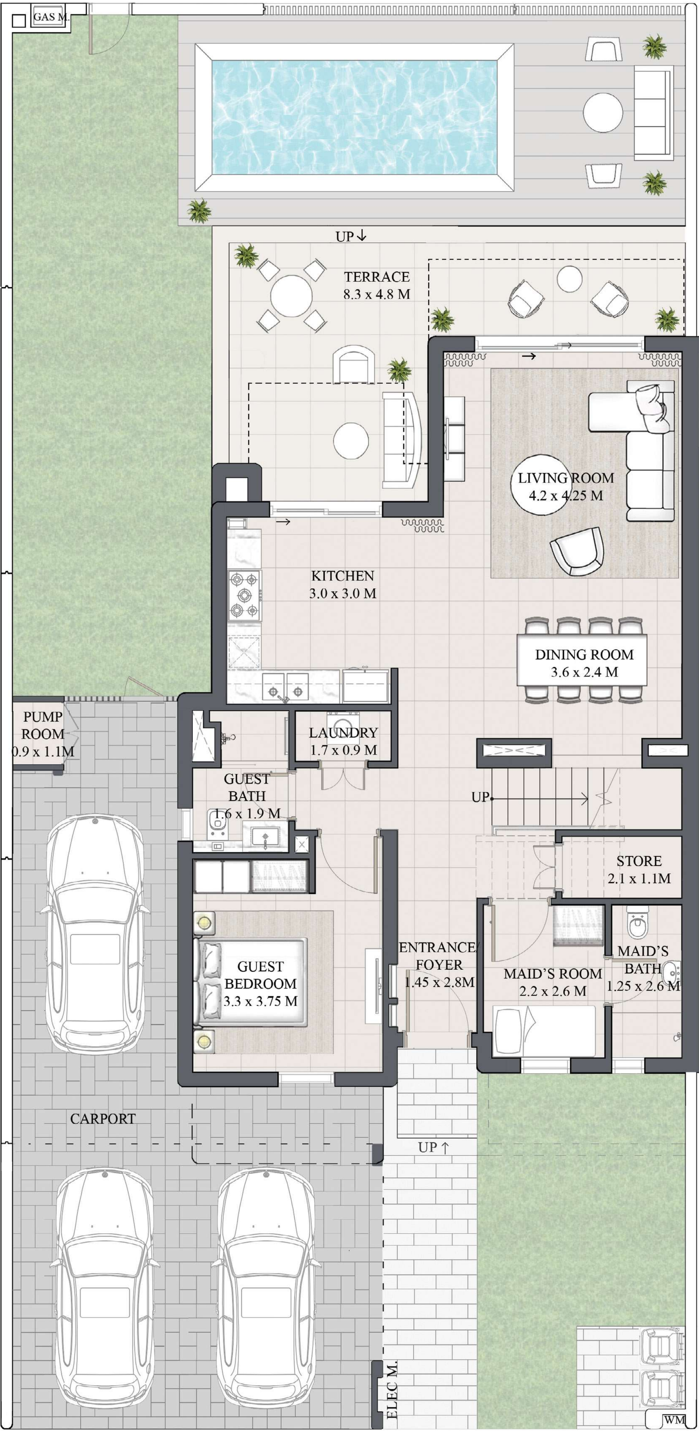
GROUND FLOOR
