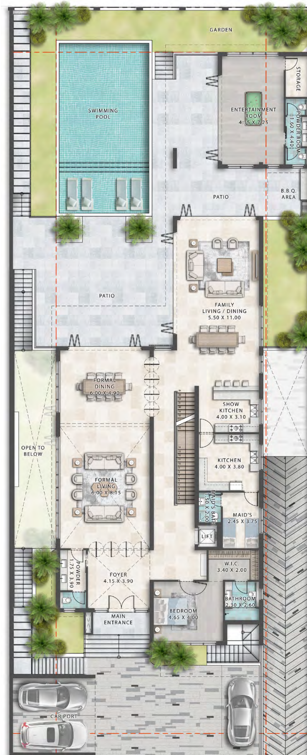
GROUND FLOOR
