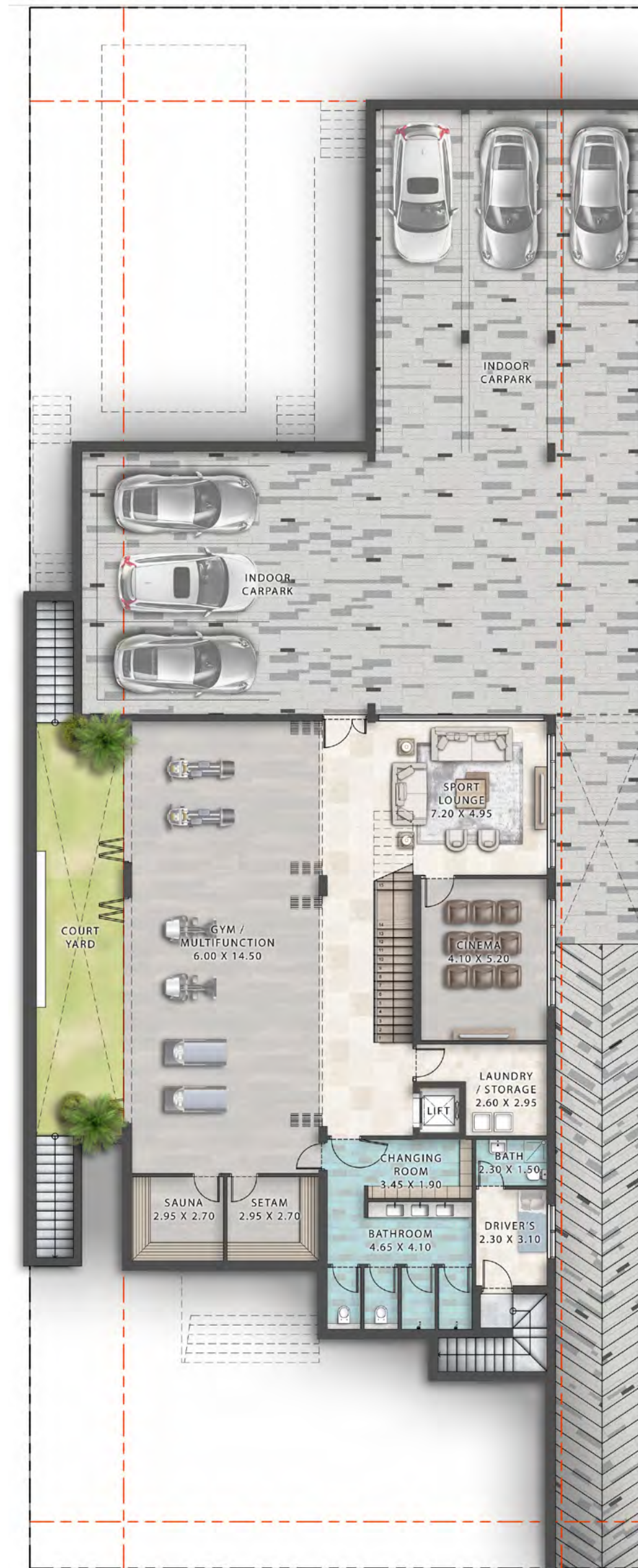
BASEMENT FLOOR
